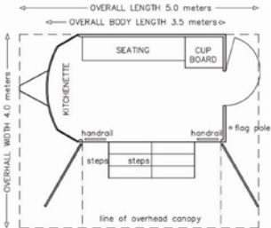
plan - unit 21
